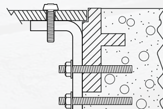
Steel Access Panel/ Grate/Vault
